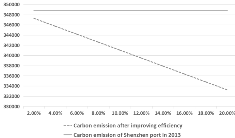
Figure 7. Carbon emissions from the Port of Shenzhen in 2013 after improving the efficiency of loading and unloading to different degrees (tons).
